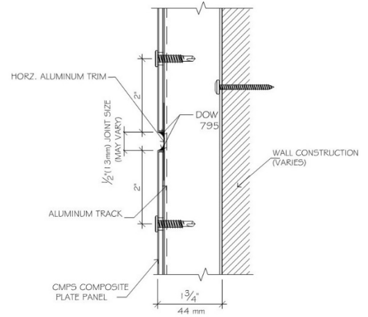
HORIZONTAL JOINT DETAIL
